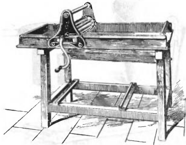
FIG. 16.—Butter-Worker.
