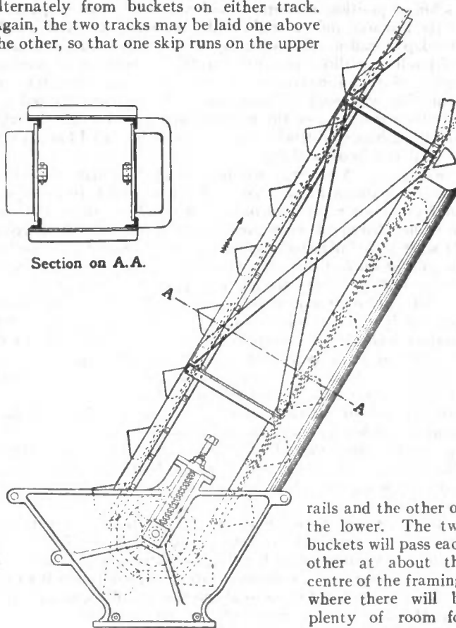
FIG. 16.—Mineral Elevator, lower terminal.
