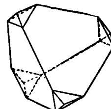
FIG. 33.—Combination of Tetrahedron and Rhombic Dodecahedron.
