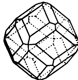
FIG. 20.—Combination of Icositetrahedron \{211\} and Rhombic Dodecahedron.
