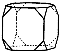
FIG. 6.—Cube in combination with Octahedron.
