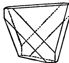
FIG. 31.—Combination of Tetrahedron and Cube.
