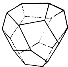
FIG. 41.—Tetrahedral Pentagonal Dodecahedron.
