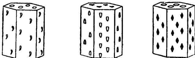
FIG. 92.—Nepheline. FIG. 93.—Calcite. FIG. 94.—Beryl. Etched Figures on Hexagonal Prisms.
