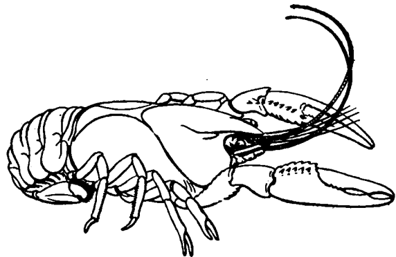
Crayfish ( Cambarus sp.) from the Mississippi River. (After Morse.)
