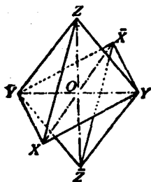
FIG. 62.—Monoclinic Axes and Hemi-pyramid.
