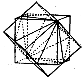
FIG. 84.—Interpenetrating Twinned Cubes.
