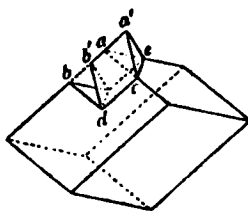
FIG. 91.—Glide-plane of Calcite.
