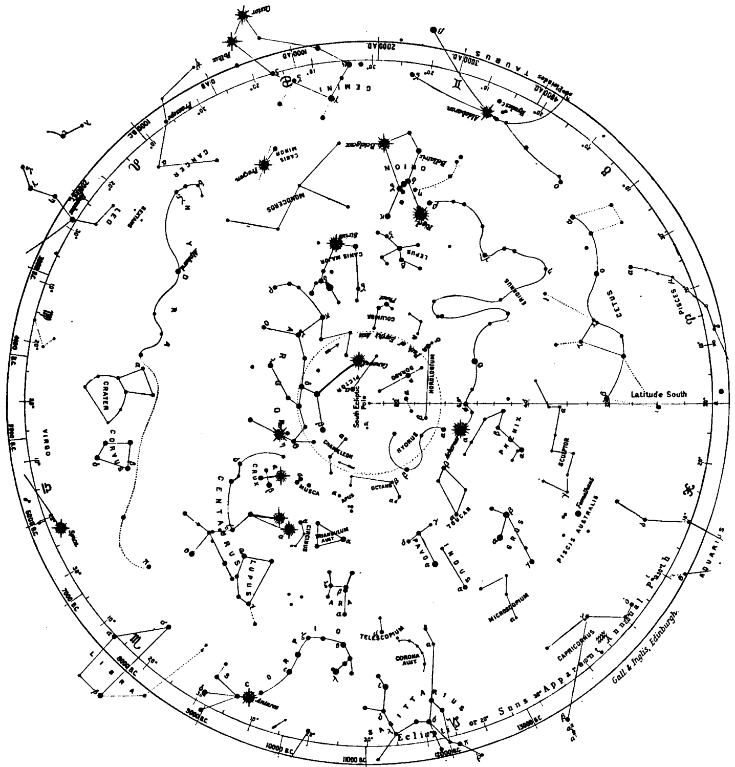
CONSTELLATIONS OF THE SOUTHERN HEMISPHERE.
