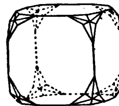
FIG. 18.—Combination of Icositetrahedron and Cube.
