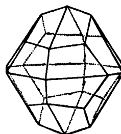
FIG. 35.—Dyakis-dodecahedron.
