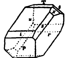
FIG. 65.—Crystal of Axinite.
