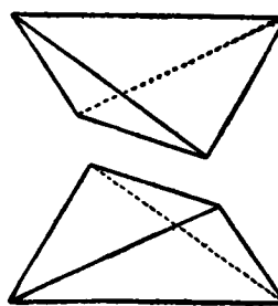
FIG. 50.—Tetragonal Bisphenoids.
