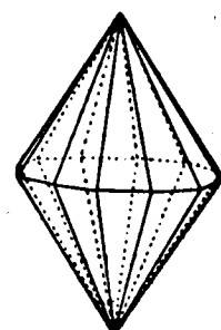
FIG. 77.—Dihexagonal Bipyramid.
