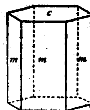
FIG. 71.—Hexagonal Prism and Basal Pinacoid.
