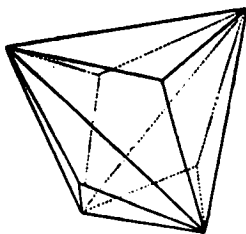
FIG. 28.—Triakis-tetrahedron.
