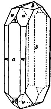
FIG. 59.—Crystal of Hypersthene.
