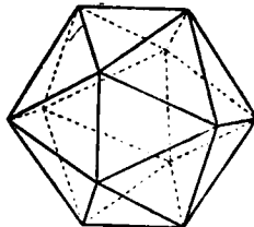
FIG. 37.—Combination of Pentagonal Dodecahedron and Octahedron.
