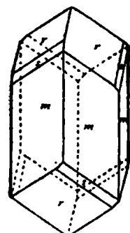
FIG. 76.—Crystal of Diopside.
