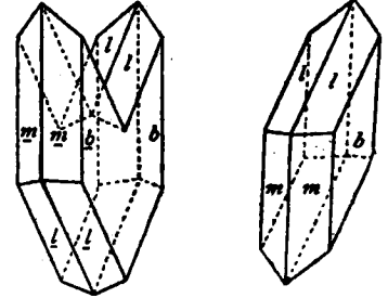
FIG. 81.—Twinned Crystal of Gypsum. FIG. 82.—Simple Crystal of Gypsum. being twinned on the plane \{100\} .
