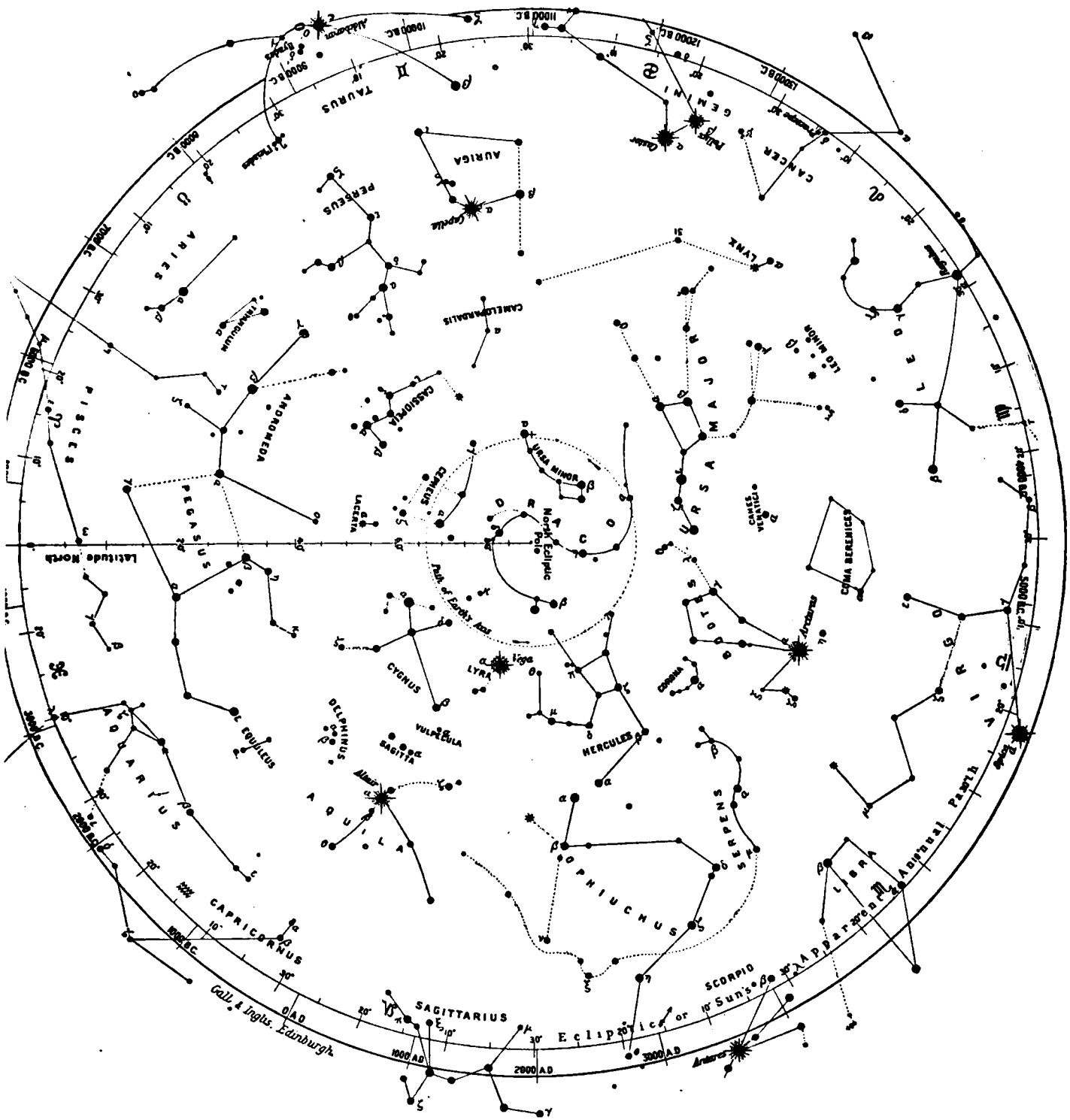
CONSTELLATIONS OF THE NORTHERN HEMISPHERE.
