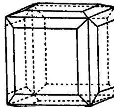
FIG. 23.—Combination of Tetrakis-hexahedron and Cube.
