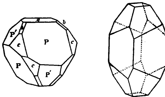
FIG. 52.—Crystal of Chalcopyrite. FIG. 53.—Crystal of Fergusonite.
