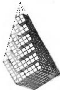
FIG. 1.—Scalenohedron built up of Rhombohedra.
