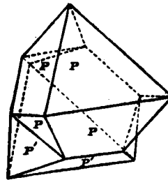
FIG. 83.—Spinel-twin.
