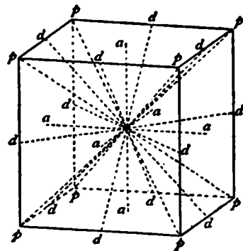
FIG. 5.—Axes of Symmetry of a Cube.
