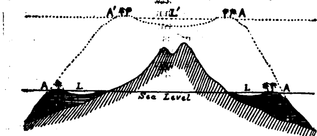
Diagram showing the formation of an atoll during subsidence. (After C. Darwin.) The lower part of the figure represents a barrier reef surrounding a central peak.
