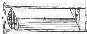
FIG. 102.—Dichroscope.
