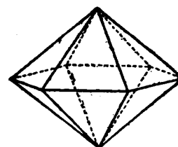
FIG. 70.—Hexagonal Bipyramid.
