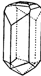
FIG. 60.—Crystal of Hemimorphite.
