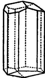
FIG. 73.—Crystal of Tourmaline.
