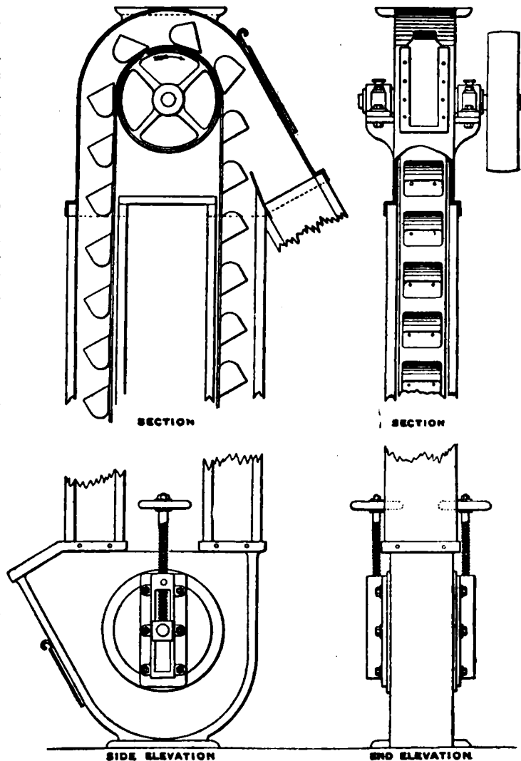
FIG. 14.—Grain Elevator.
