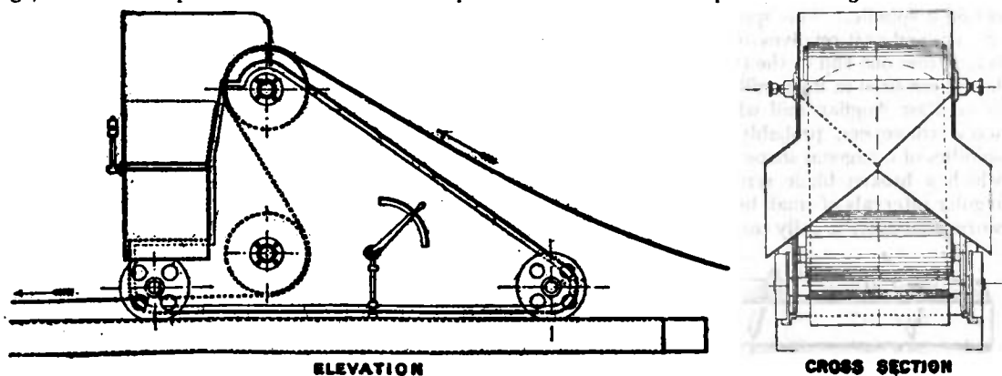
FIG. 6.—Throw-off Carriage for Band Conveyor.
